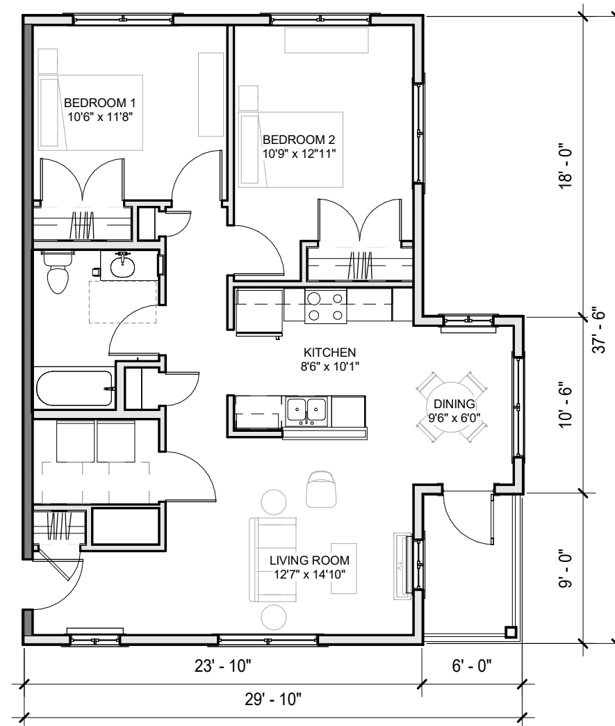
① GARDEN - 2 BED 1/8" = 1'-0"
