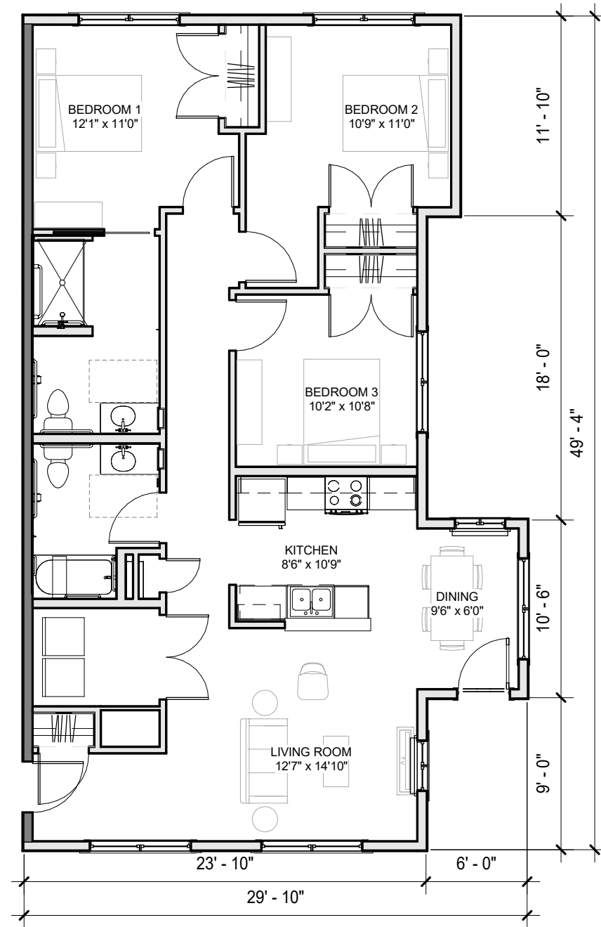
① GARDEN - 3 BED 1/8" = 1'-0"
