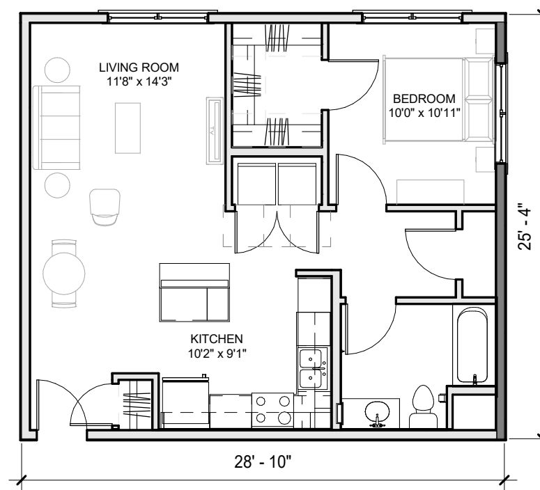
① WALK-UP APARTMENT - 1 BED 1/8" = 1'-0"
