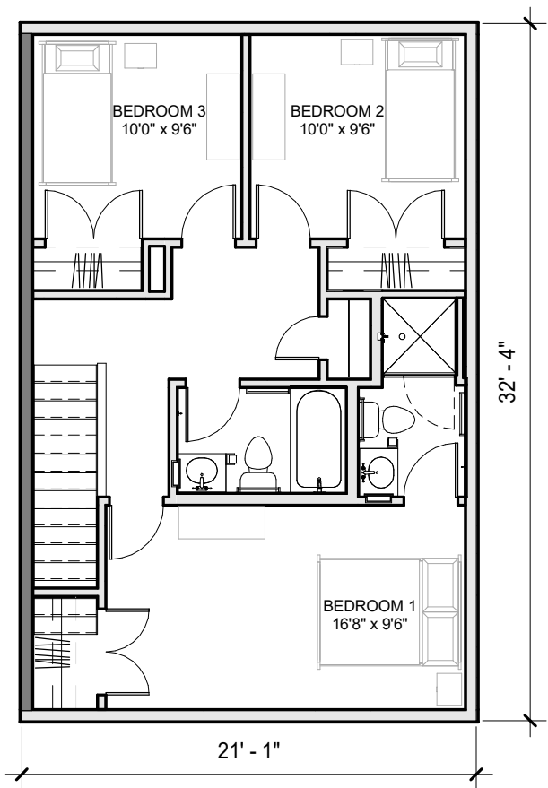
② TOWNHOUSE - 3 BED SECOND FLOOR 1/8" = 1'-0"
