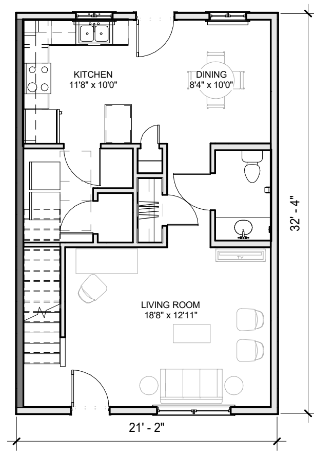
① TOWNHOUSE - 3 BED FIRST FLOOR 1/8" = 1'-0"
